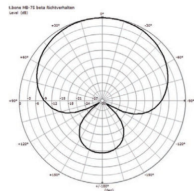
Polar pattern @ 1 kHz
