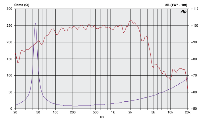
*2.83V. Half space response measured in a 107 Litre vented enclosure.
