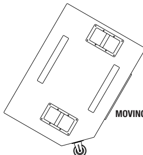
MOVING POSITION CARTWHEELS Art. 37223 / 37224
