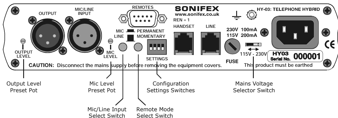
Figure 2-2 : Rear Panel Controls
