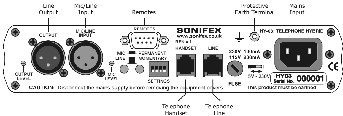
Figure 3-1 : HY-03 Rear Panel Connections
