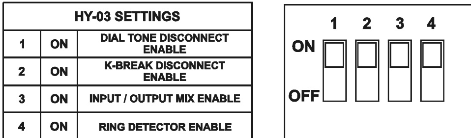
Figure 2-3 : Configuration Settings Switches
