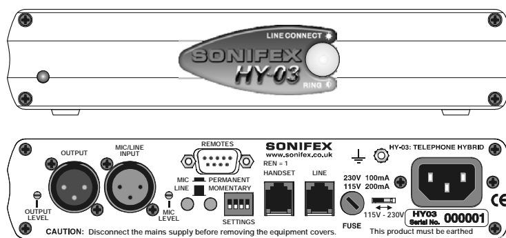
Figure 1-1 : HY-03 & HY-03 US Front & Rear
