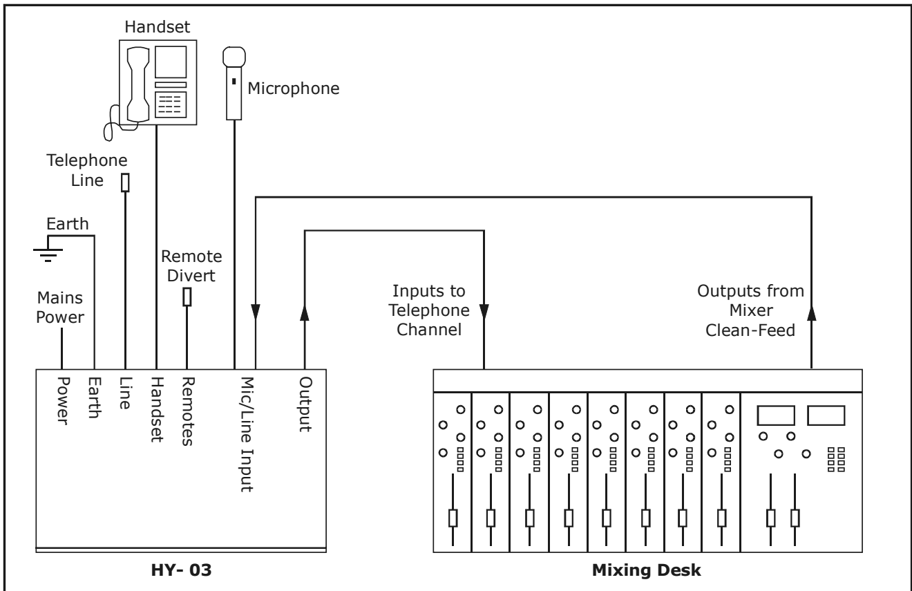
Figure 1-4 : HY-03 User Connections
