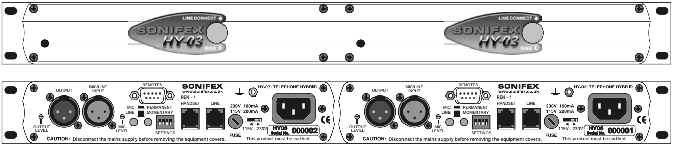
Figure 1-3 : HY-03T & HY-03T US Front & Rear
