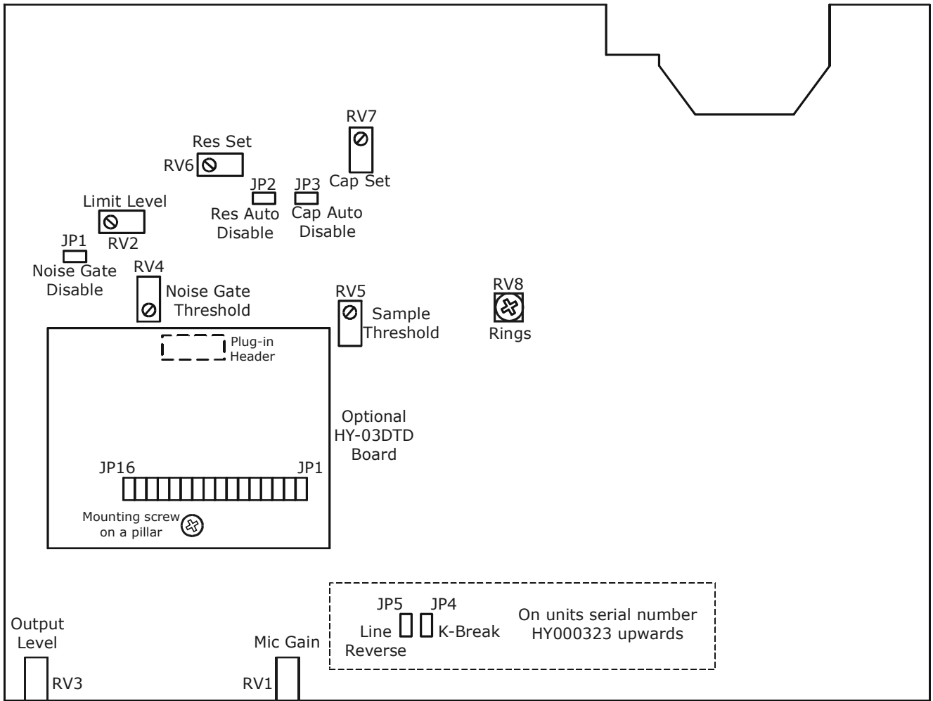
Figure 2-4 : HY-03 Preset Controls and Alignments
