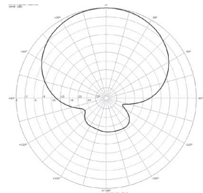
Polar pattern @ 1 kHz
