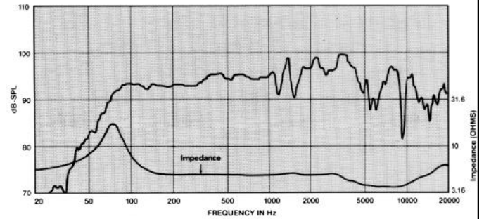
Frequency Response, 1 W at 1 m; Impedance
